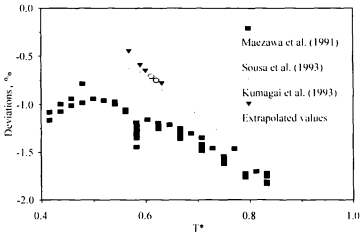
Fig. 1. Deviations of the density of HCFC 141b from the values predicted by the RHSDS. Deviations = (\rho_{\text{exp}} - \rho_{\text{RHSDS}}) / \rho_{\text{RHSDS}} \times 100 .
